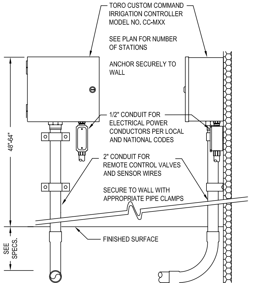
FRONT SECTION/ELEVATION NOT TO SCALE
