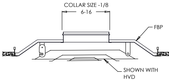
FBP Typical Installation
