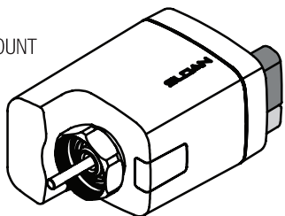
EBV-505-A SLEEVE ASSEMBLY (SUPPLIED WITH HEX WRENCH)
