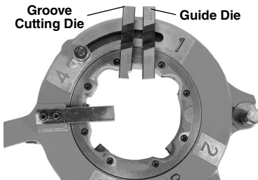
Figure 2 – Inserting Dies
