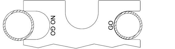
Figure 3 – Sertissage conforme
