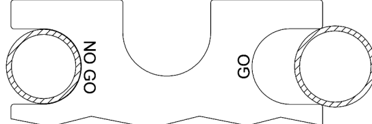
Figure 2 – Out of Tolerance Connections
