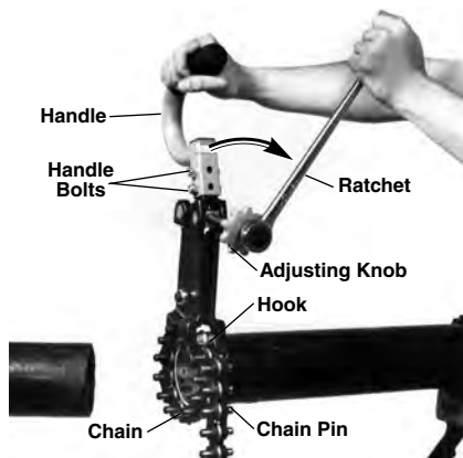
Figure 4 – Using the 226 Soil Pipe Cutter
