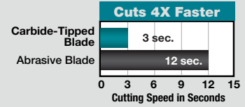
Carbide Abrasive
