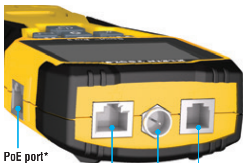
RJ45 port*
