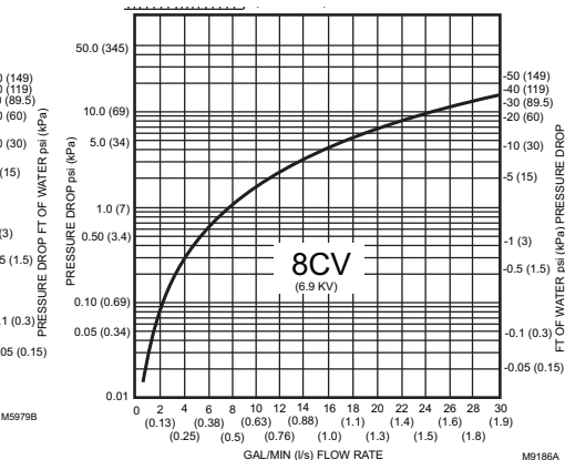
Fig. 2c. Flow characteristics of 8 Cv (6.9 kV) valve.
