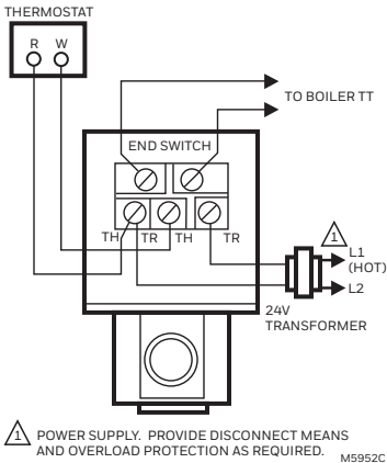
Fig. 5. Typical wiring for V8043F.
