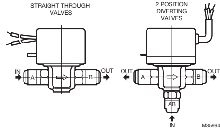
Fig. 2. Inlet and outlet ports on straight-through and diverting valves.
