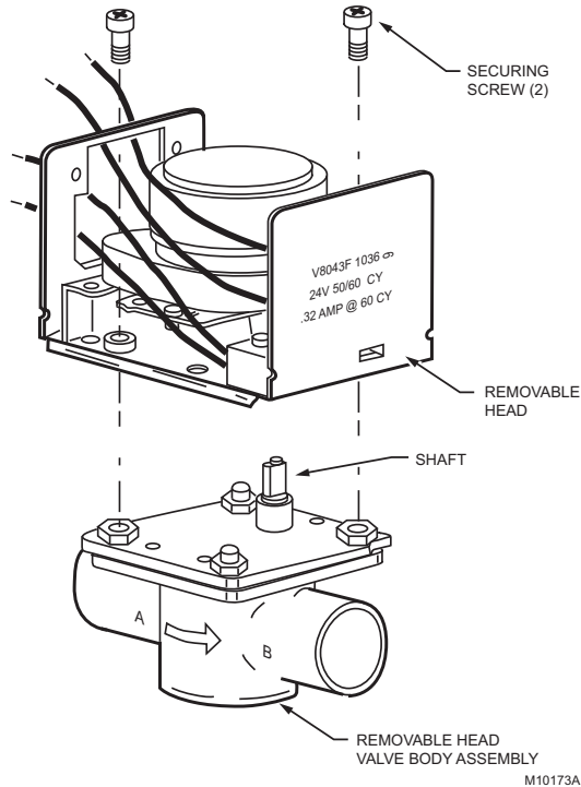
Fig. 12. Install new powerhead.
