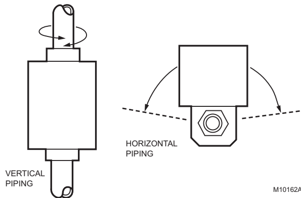
Fig. 9. Mounting positions.
