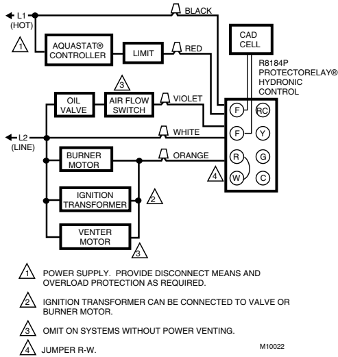
Fig. 8. Typical hydronic hookup for R8184P.
