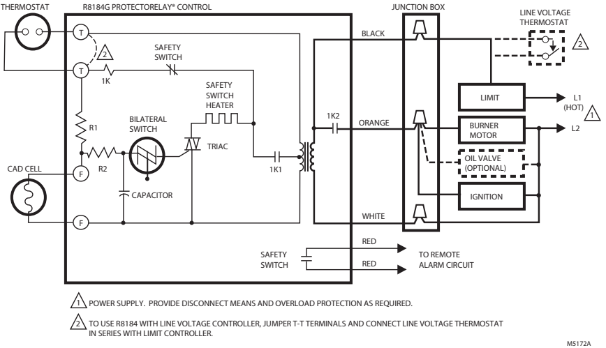
Fig. 5. Typical hookup for R8184G with dry contacts for remote alarm.
