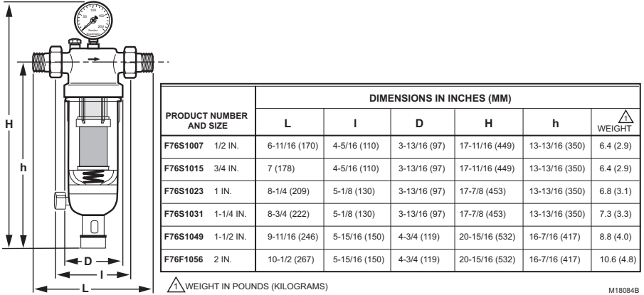
Fig. 1. F76S Dimensions.
