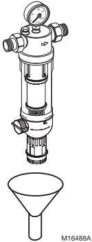
Fig 2a. Ideal F76S installation. A funnel mounted directly under the backwash port is the best installation layout.
