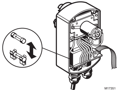
Fig. 10. Replacing the MV876 fuse.
