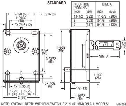
Fig. 6. L4064 Dimensions.
