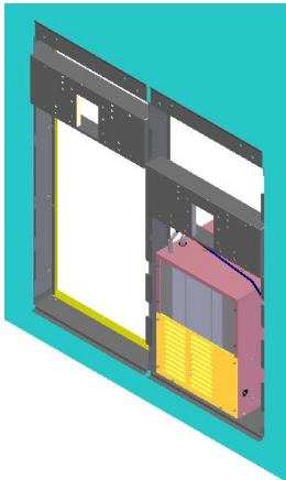
Figure 2 - Chiller Installation
