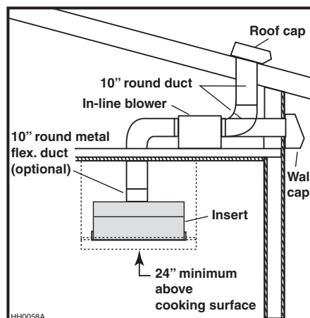
MODEL HLB3, HLB6, HLB9 OR HLB11 IN-LINE BLOWER TYPICAL DUCTWORK
