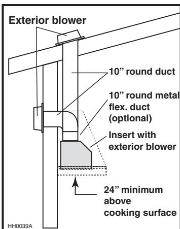
MODEL 331H, 332H, 335 OR 336 EXTERIOR BLOWER TYPICAL DUCTWORK
