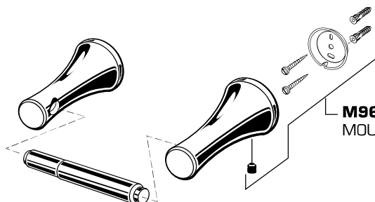
TOILET PAPER HOLDER 8337.230
