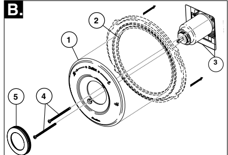
Escutcheon Installation for Models T14053, T14253, T14453, T14067, T14267 & T14467.
