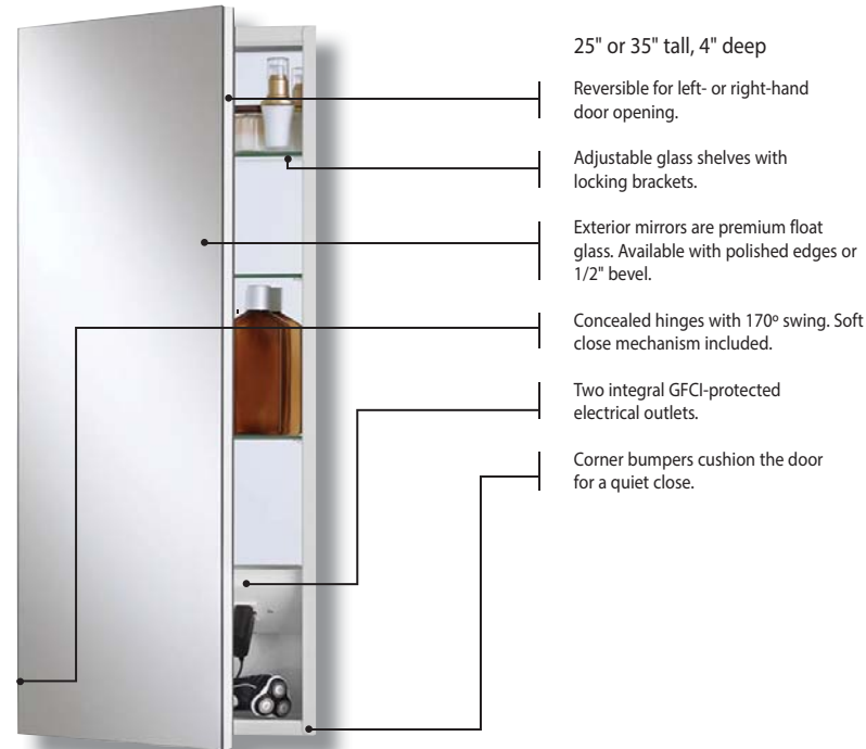
Meridian - Electric 704325 Cabinets can be mounted in tandem vertically and horizontally. *Ganging Kits required, see pg. 42)
