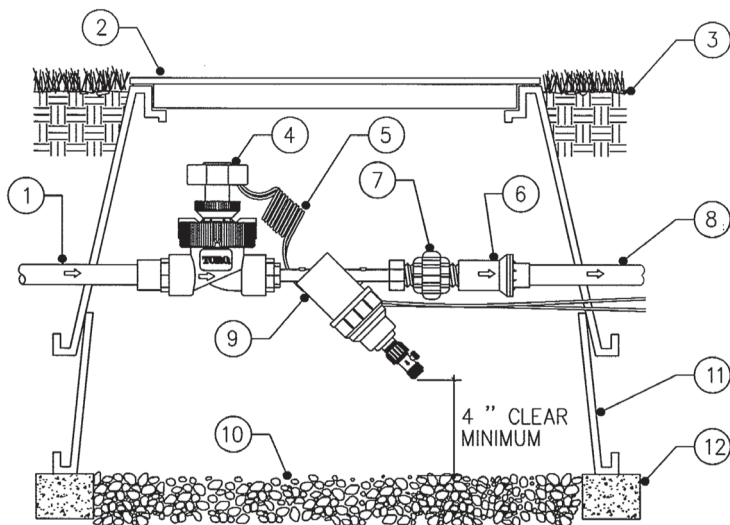
SECTION/ELEVATION
