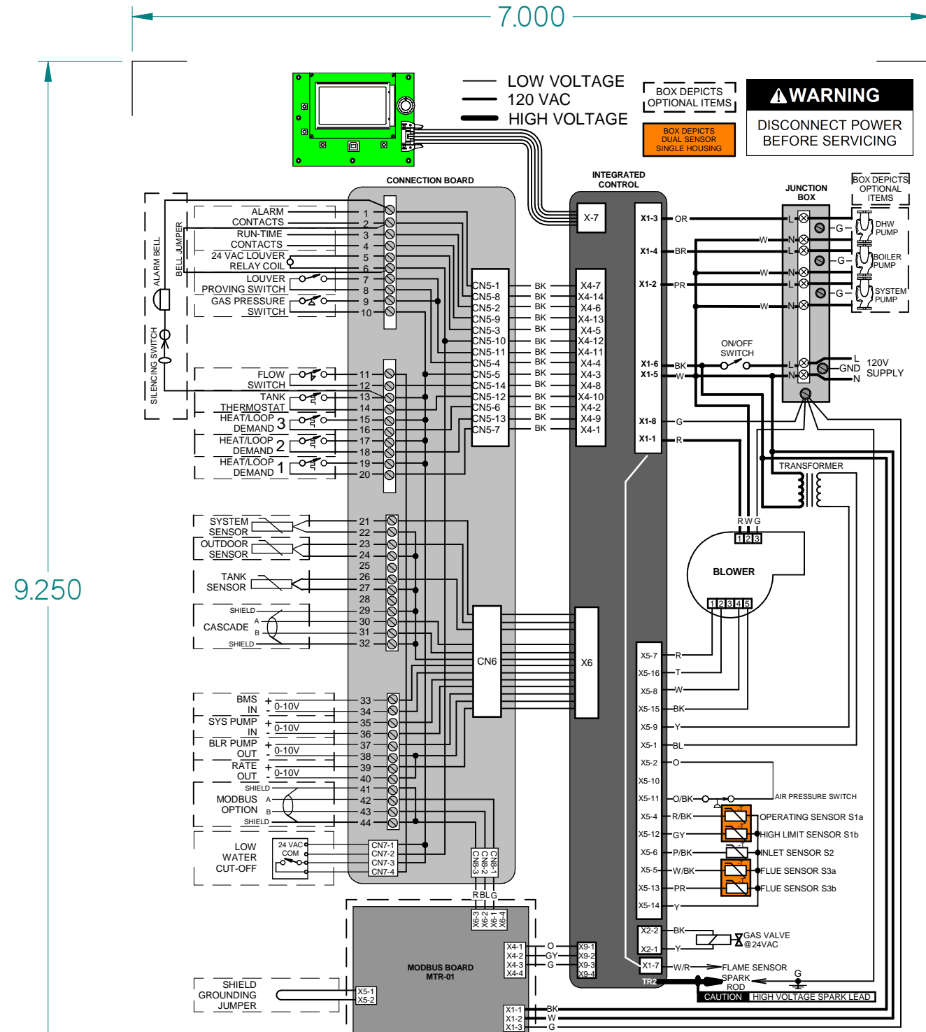
WIRING DIAGRAM LBL20169 REV C
