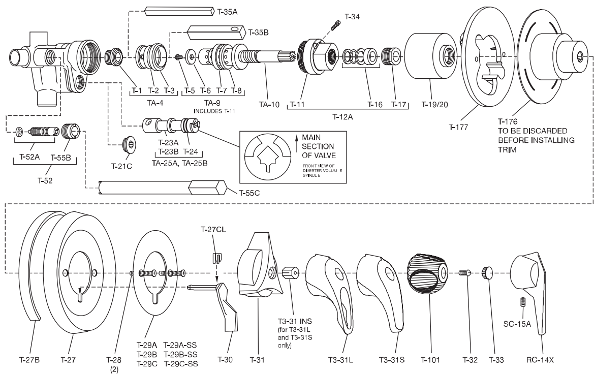
FIGURE 9 Parts Breakdown
