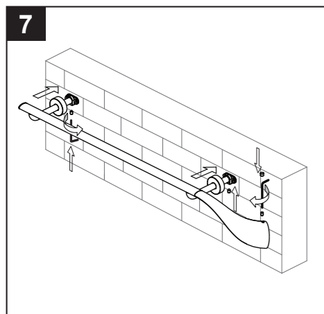
7 Place towel bar assembly on the mounting brackets. Secure it to the wall using the bottom set screws.
