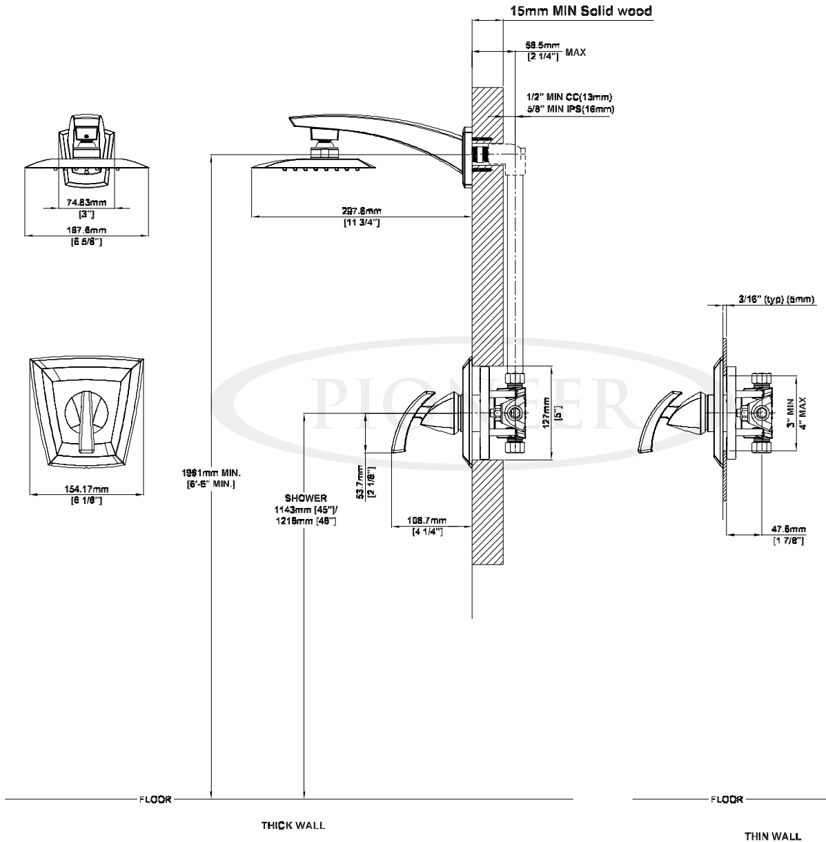
Product Diagram
