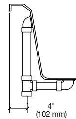
PLUMBING ROUGH-IN
