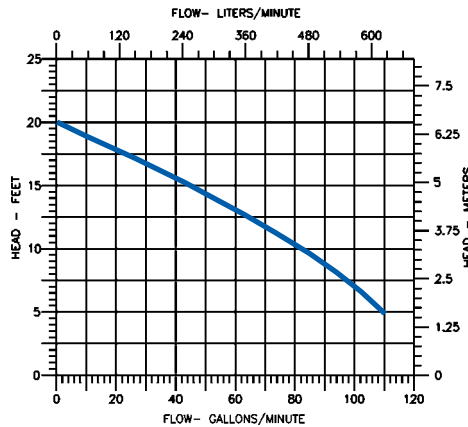
10S Series Pump Performance Curve
