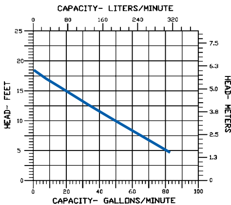
9S Series Pump Performance Curve
