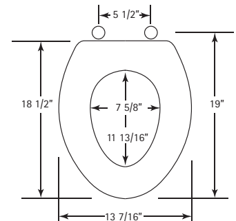
Ring thickness is 5/8" Ring thickness including the bumper is 1-3/16"
